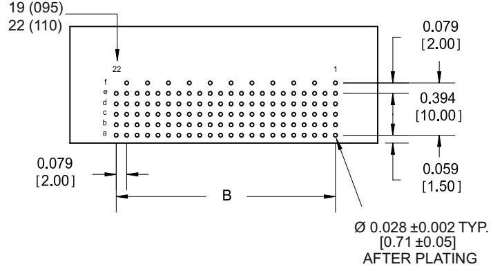
Component side of PCB
