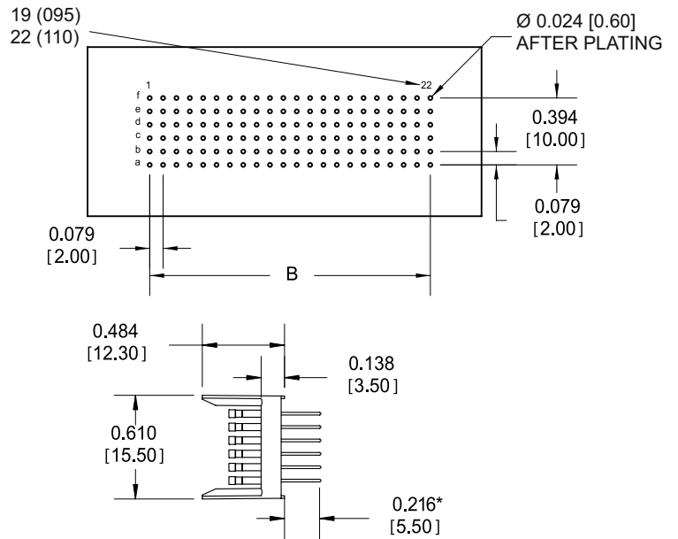
Component side of PCB
