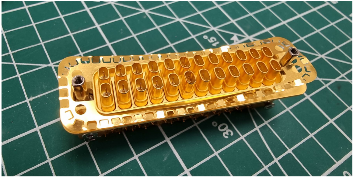
Nexus Connector – with EMC gasket
