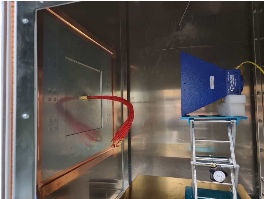
Test setup – Plug side
