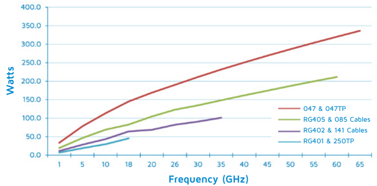
Attenuation vs Frequency
