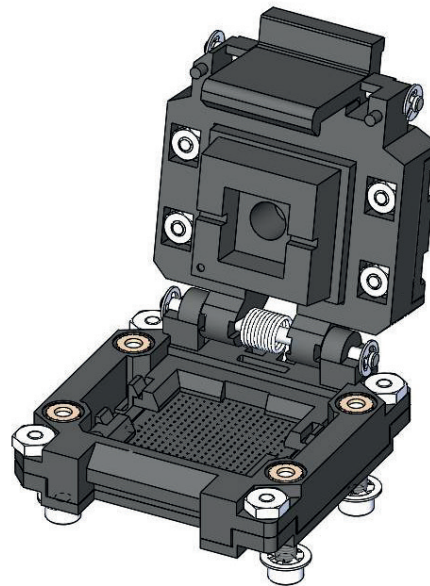
Spring-loaded plunger
