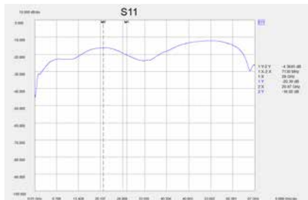
Return Loss
