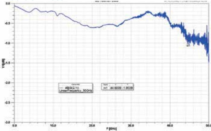
Insertion Loss
