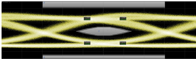
Typical optical eye of LightABLE 28G LL (6.5 ps per division)
