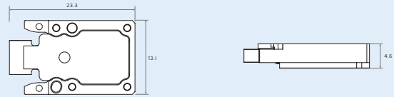
Actual size of LightABLE 10G LL 4TRX, 12TX, and 12RX*
