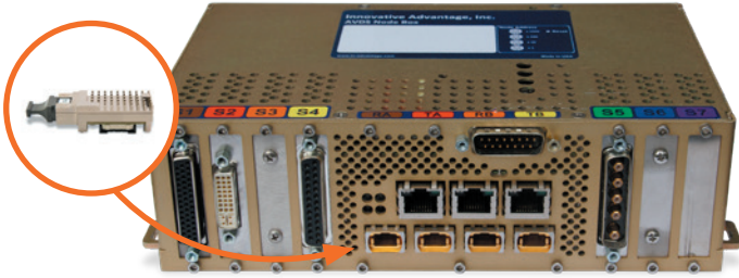
AVDS node for IFE applications use SNAP12 transceivers.
