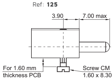
Unpolarised transverse mount (moulding A)
