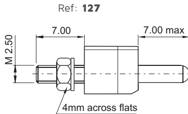
Unpolarised vertical mount (moulding B)
