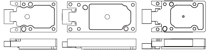
Real size for SpaceABLE 10G SL Series 4TRX, 12TX, and 12RX (left), SpaceABLE 10G SL Series 12TRX (center), and SpaceABLE 28G 4TRX (right).
